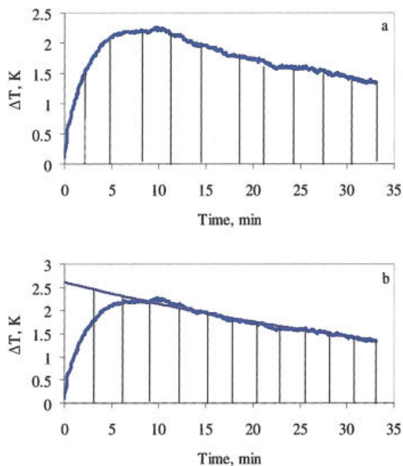
Figure 3. Area underneath the isoperibolic ΔT curve of run 7: (a) A 1 ; (b) A 2 .
